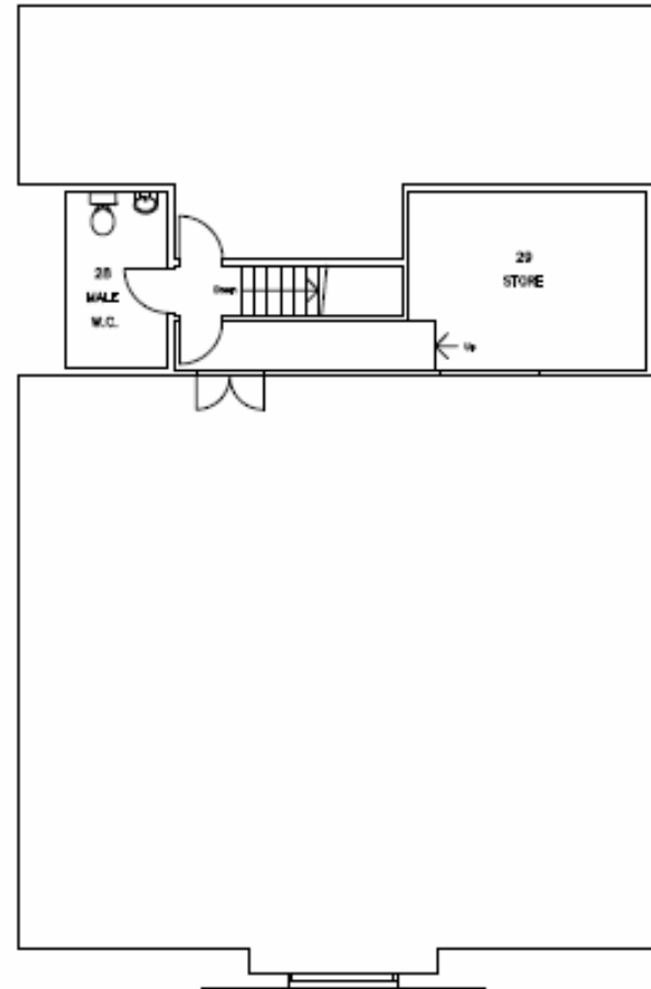
ATTIC FLOOR
