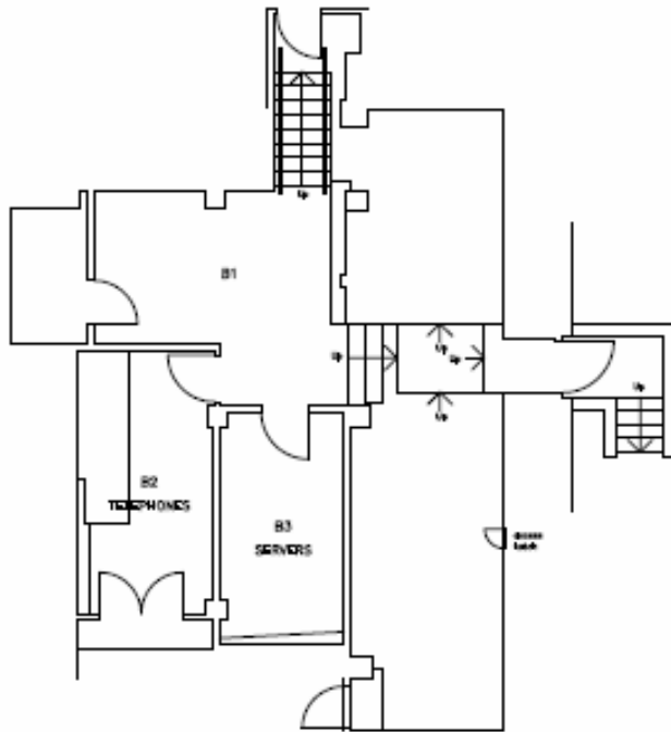
BASEMENT FLOOR
