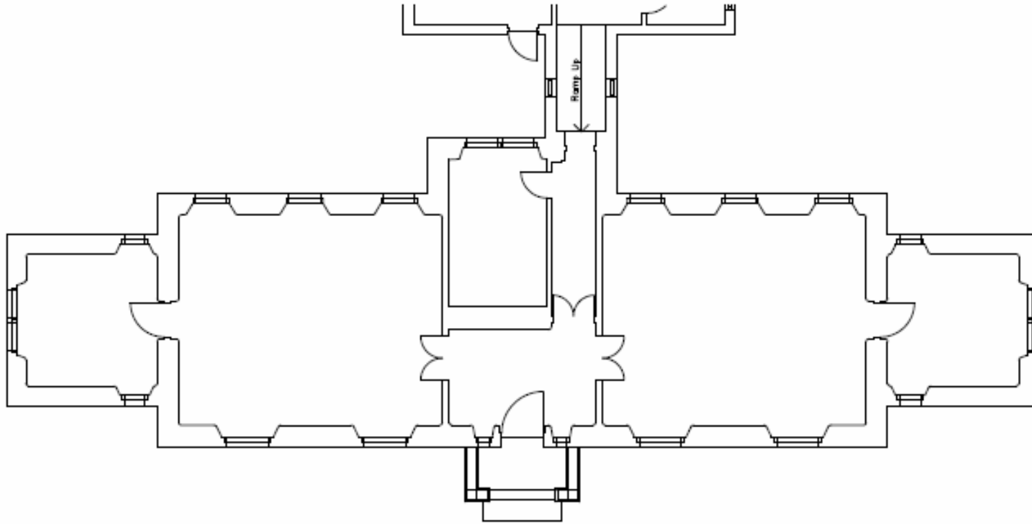
NEWSTEAD OFFICES BLOCK 2 GROUND FLOOR PLAN
