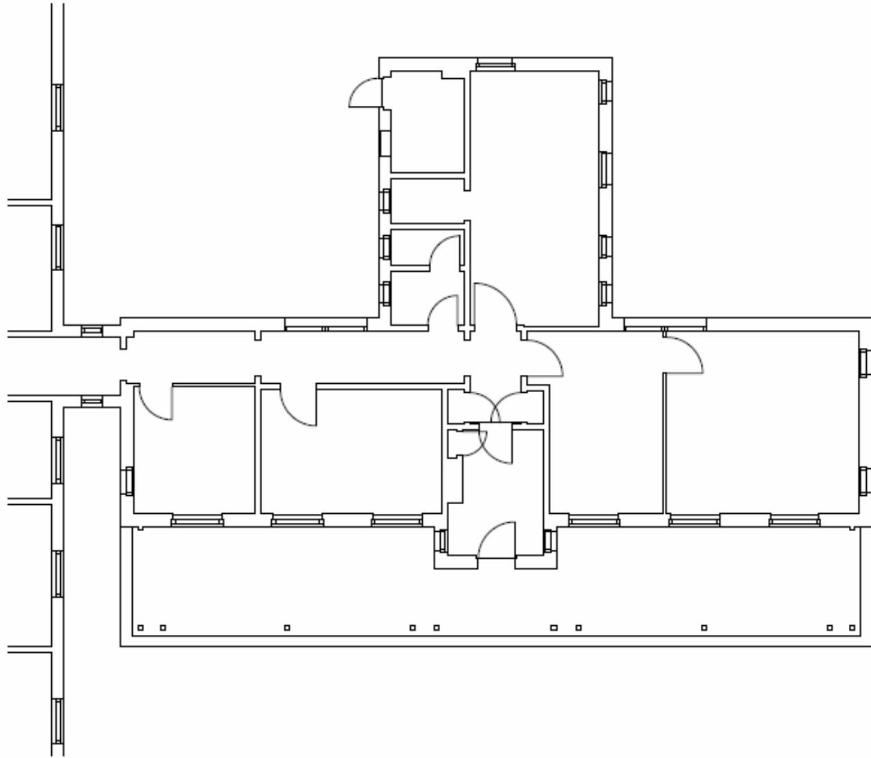
NEWSTEAD OFFICES BLOCK 3 GROUND FLOOR PLAN
