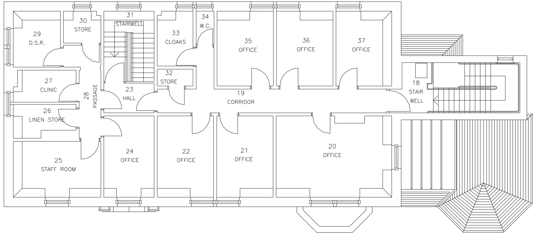
FIRST FLOOR PLAN GALA VALE – WEST BRIG
