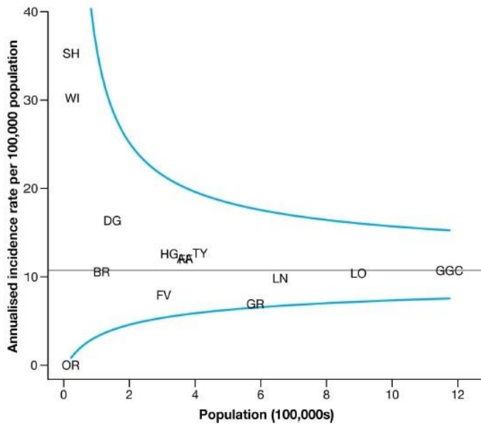
Funnel plot of SAB incidence rates (per 100,000 population) in community associated infection cases for all NHS boards in Scotland in Q1 2019. 1,2
