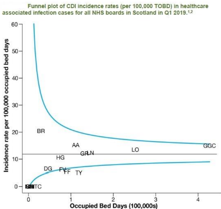
Figure 6: Funnel plot of CDI incidence rates (per 100,000 TOBD) in healthcare associated infection cases for all NHS Boards in Scotland in Q1 2019
