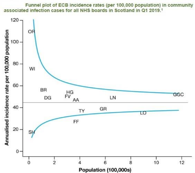
Figure 11: Funnel plot of ECB incidence rates (per 100,000 population) in community associated infection cases for all NHS Boards in Scotland in Q1 2019
