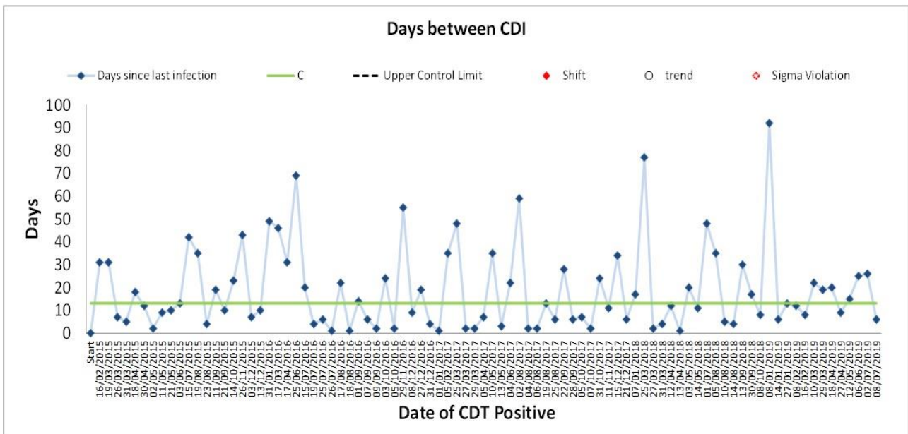
Figure 5: NHS Borders days between CDI cases (January 2015 – July 2019)
