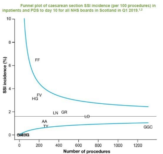
Figure 8: Funnel plot of caesarean section SSI incidence (per 100 procedures) in inpatients and Post Discharge Surveillance (PDS) to day 10 for all NHS Boards in Scotland in Q1 2019
