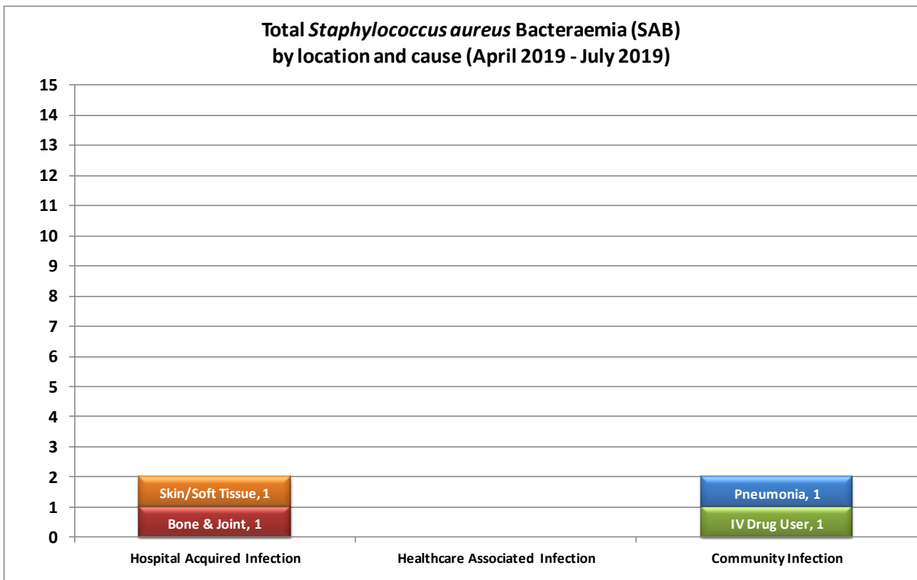
Figure 1: SAB cases by location and cause (April 2019 – July 2019)
