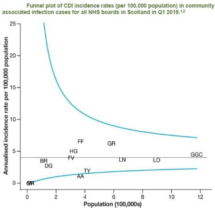
Figure 7: Funnel plot of CDI incidence rates (per 100,000 population) in community associated infection cases for all NHS Boards in Scotland in Q1 2019
