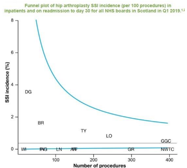
Figure 9: Funnel plot of hip arthroplasty SSI incidence (per 100 procedures) in inpatients and on readmission to day 30 for all NHS Boards in Scotland in Q1 2019
